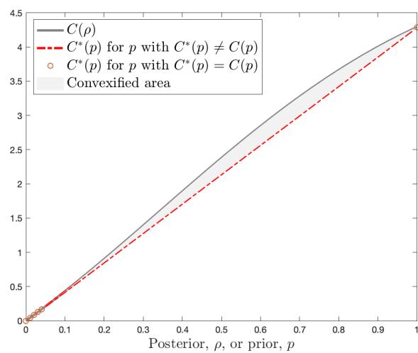
(b) Example 2: non-convex C .
