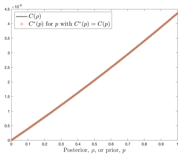
(a) Example 1: convex C .
